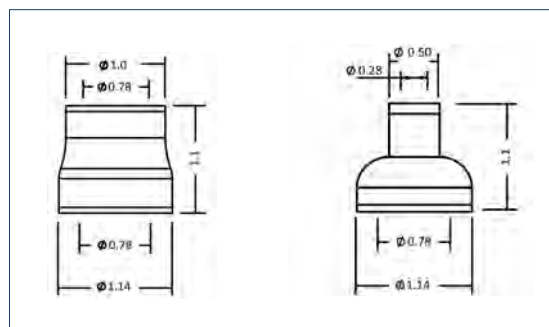
ZC050-1SWC-304 1" STANDOFF - WALL TO COMPONENT UP TO 3/4" THREAD
